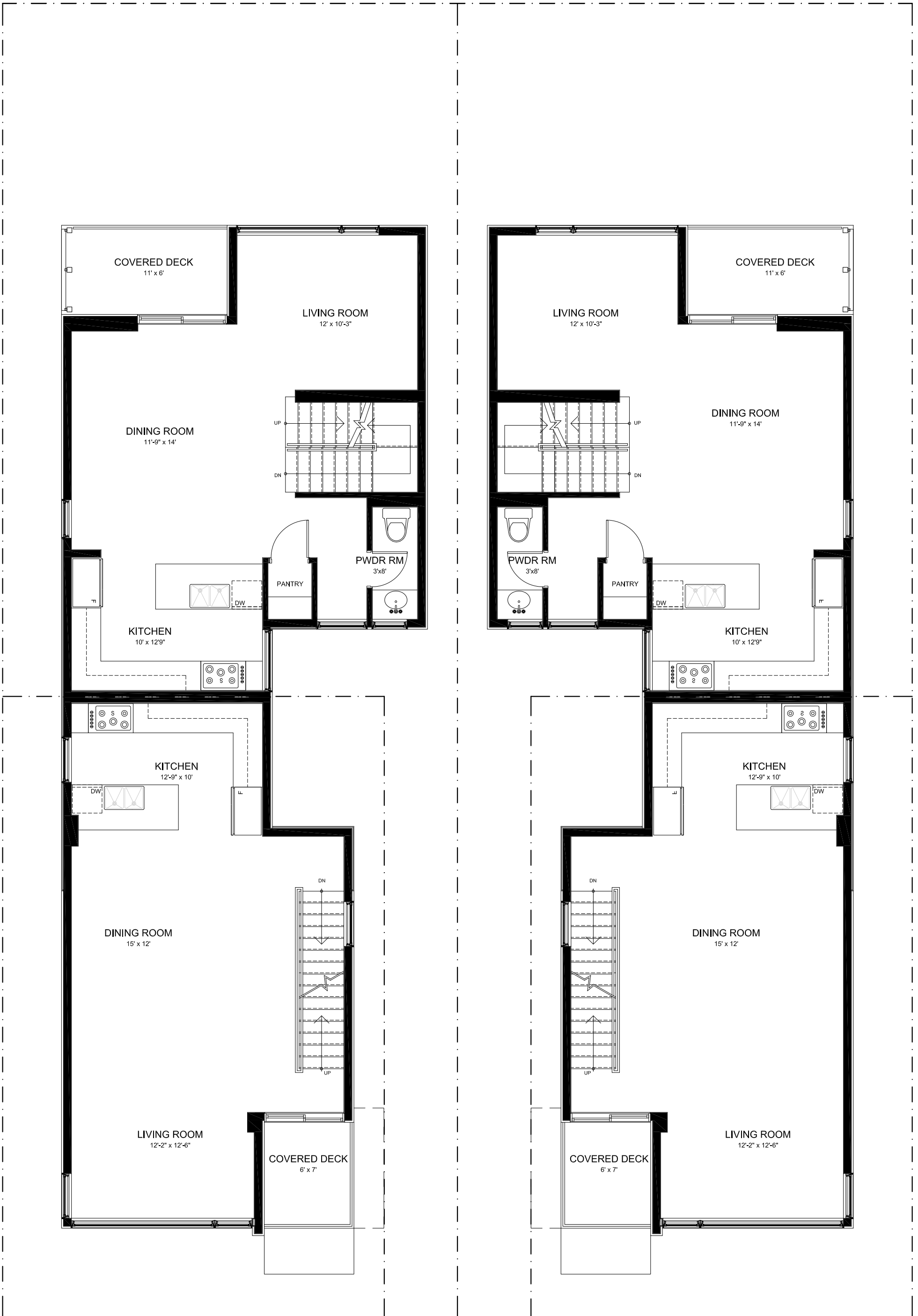
SECOND FLOOR PLAN FRONT UNIT 605 SF BACK UNIT 659 SF
