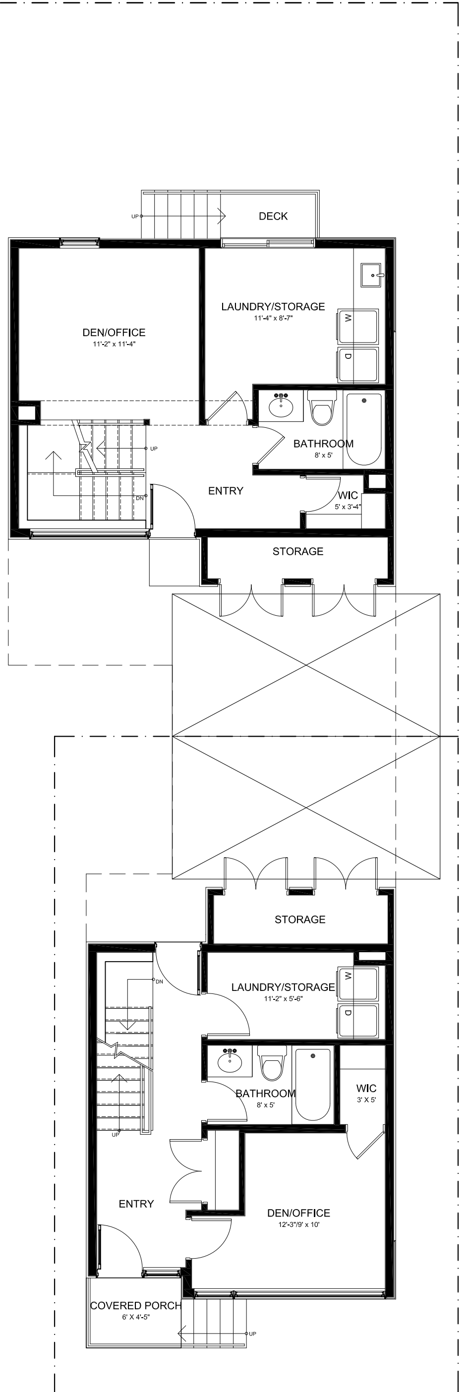
GROUND FLOOR PLAN FRONT UNIT 432 SF BACK UNIT 446 SF
