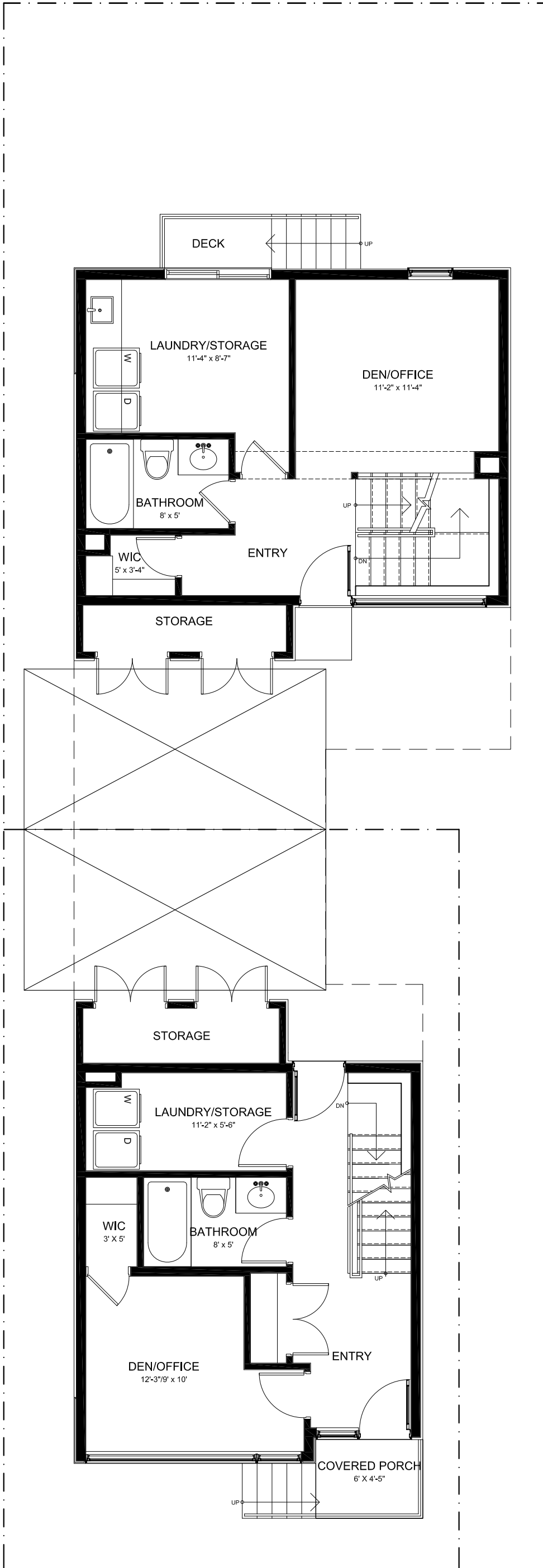
GROUND FLOOR PLAN FRONT UNIT 432 SF BACK UNIT 446 SF
