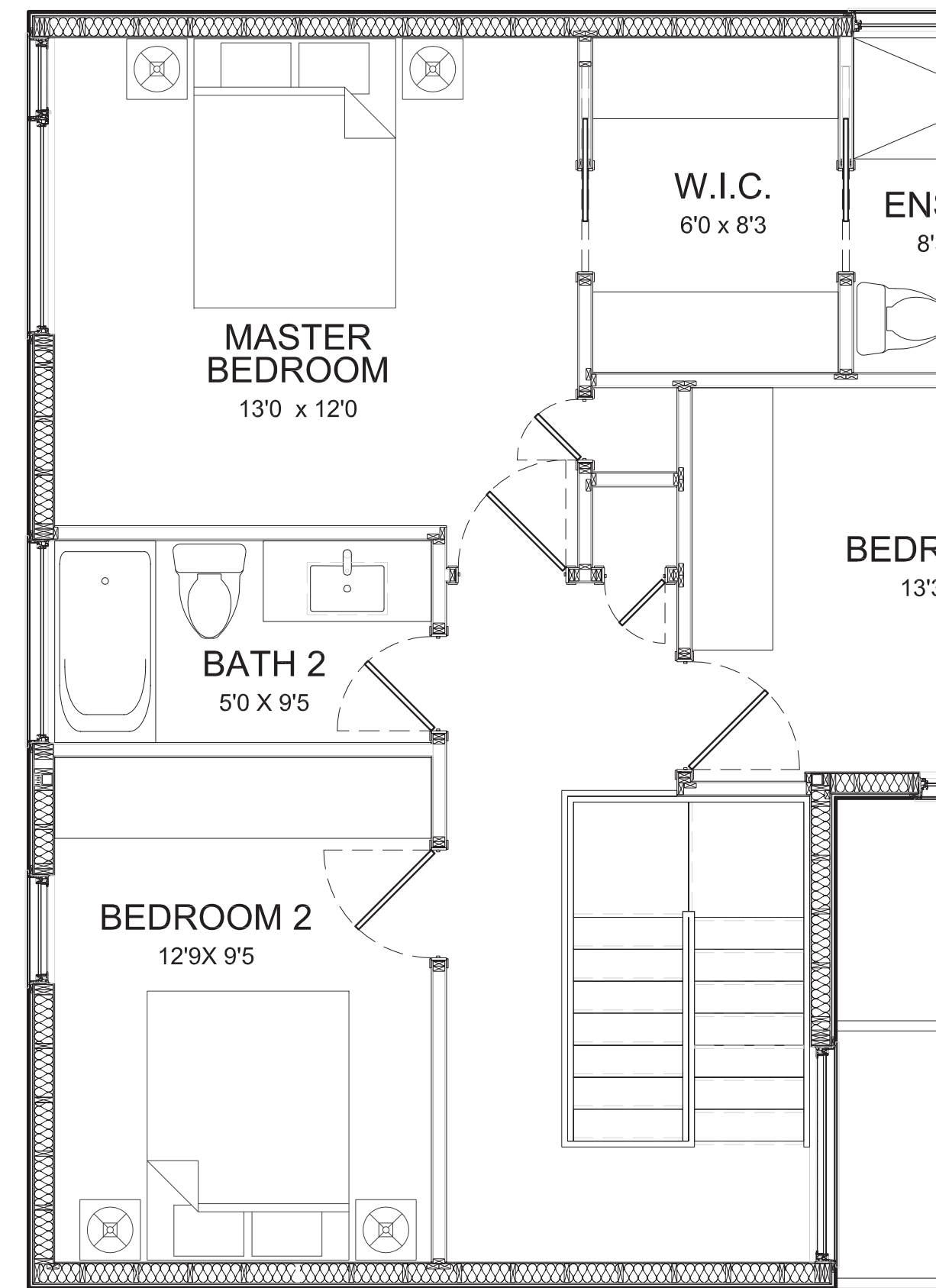
THIRD FLOOR PLAN - 782 SQ.FT.
