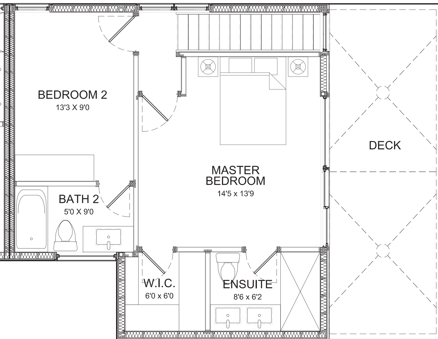
THIRD FLOOR PLAN - 563 SQ.FT.
