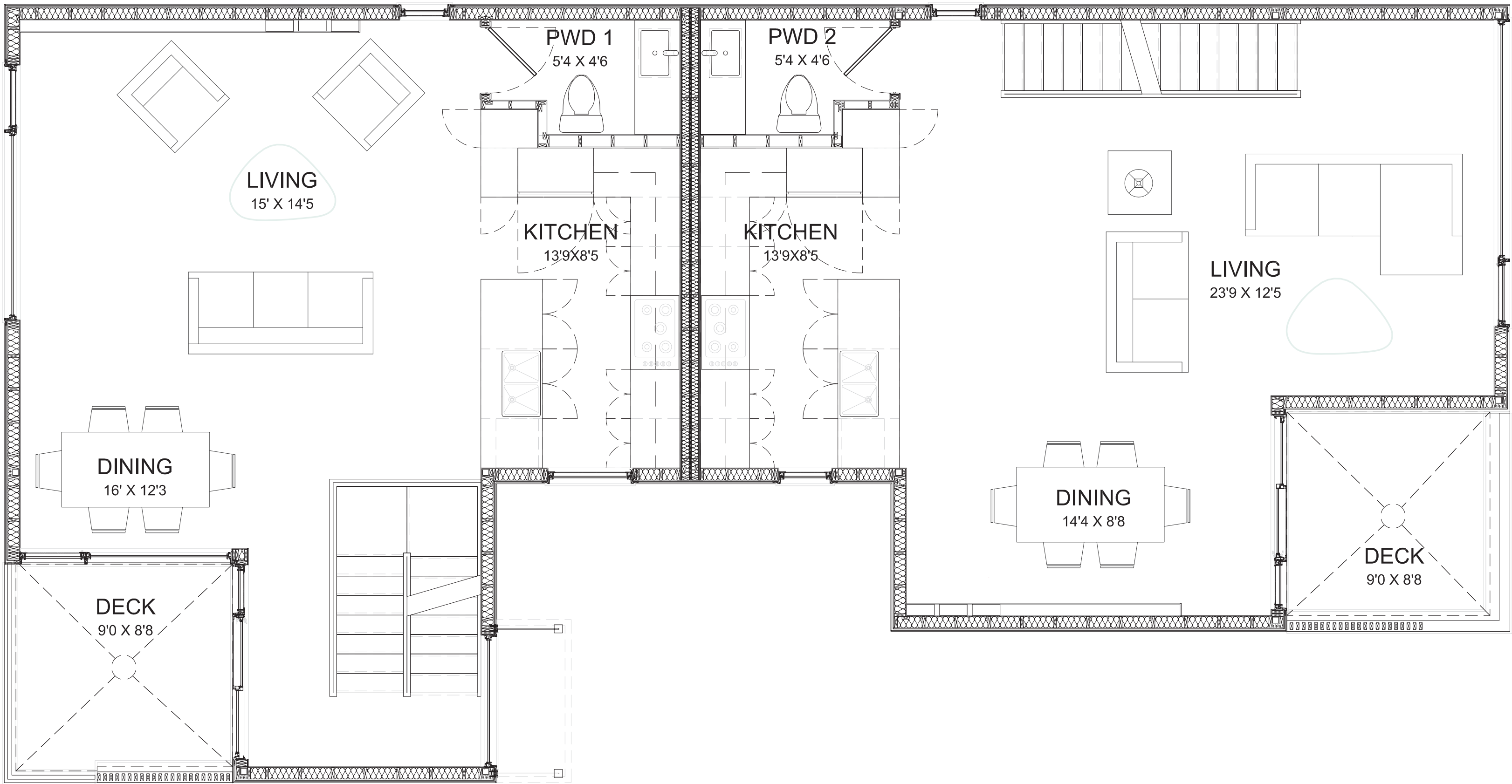
SECOND FLOOR PLAN - 714 SQ.FT.
